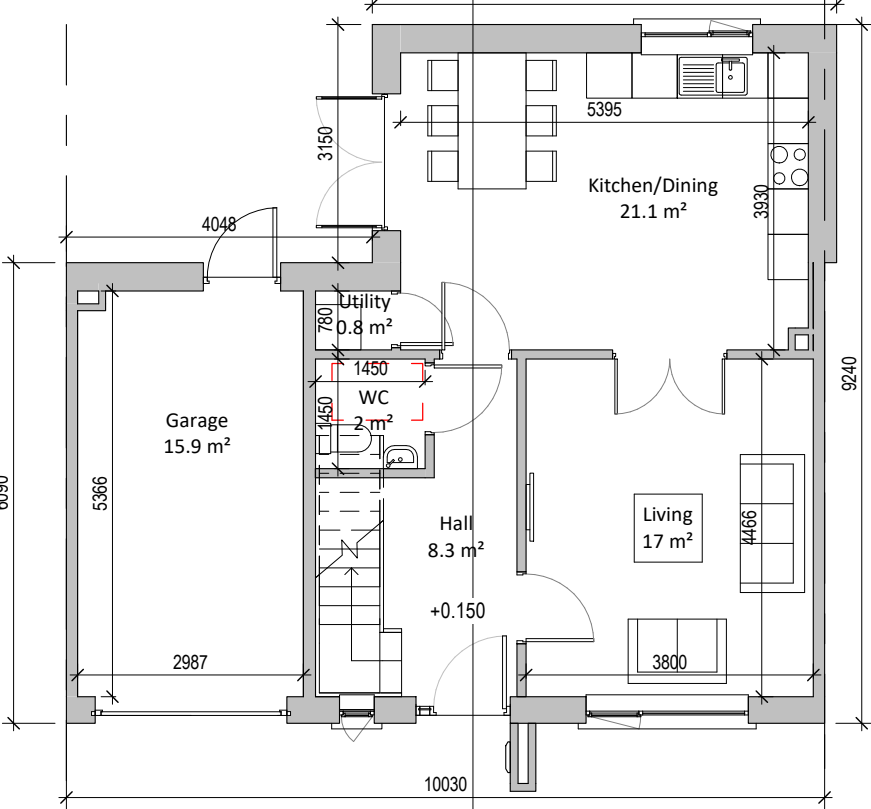
① Ground Floor Mid Terrace 1 : 100
