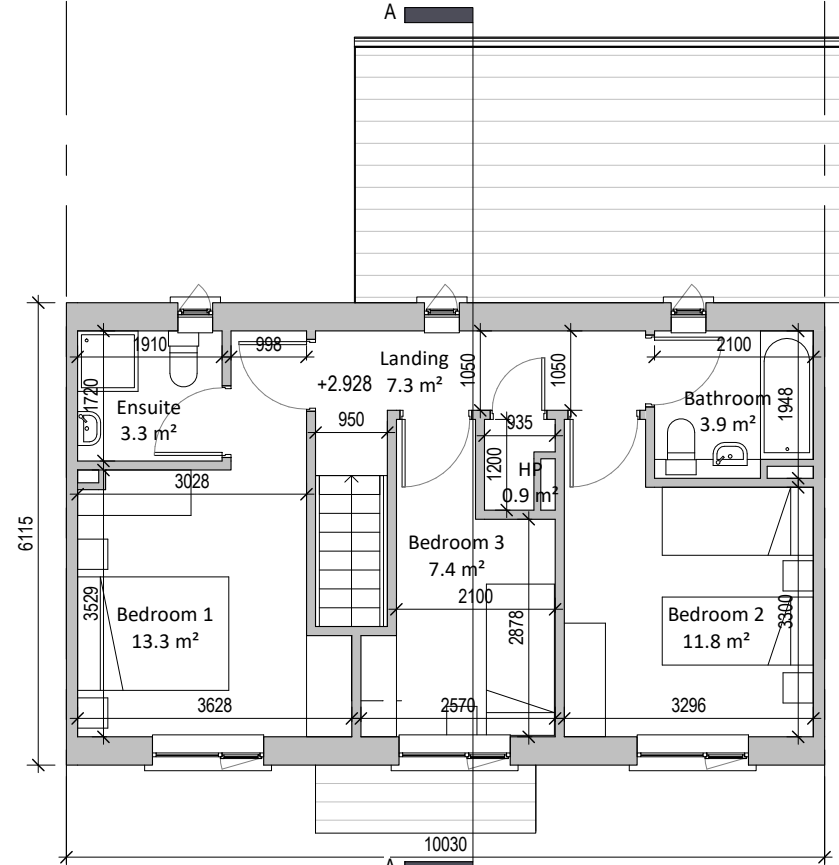
② First Floor Mid Terrace 1 : 100
